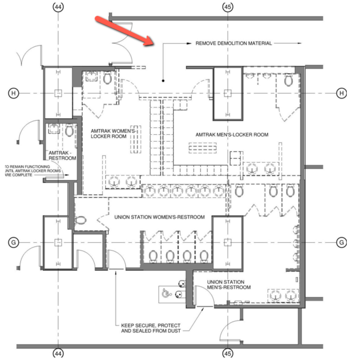
AMTRAK Locker Room Corridor
