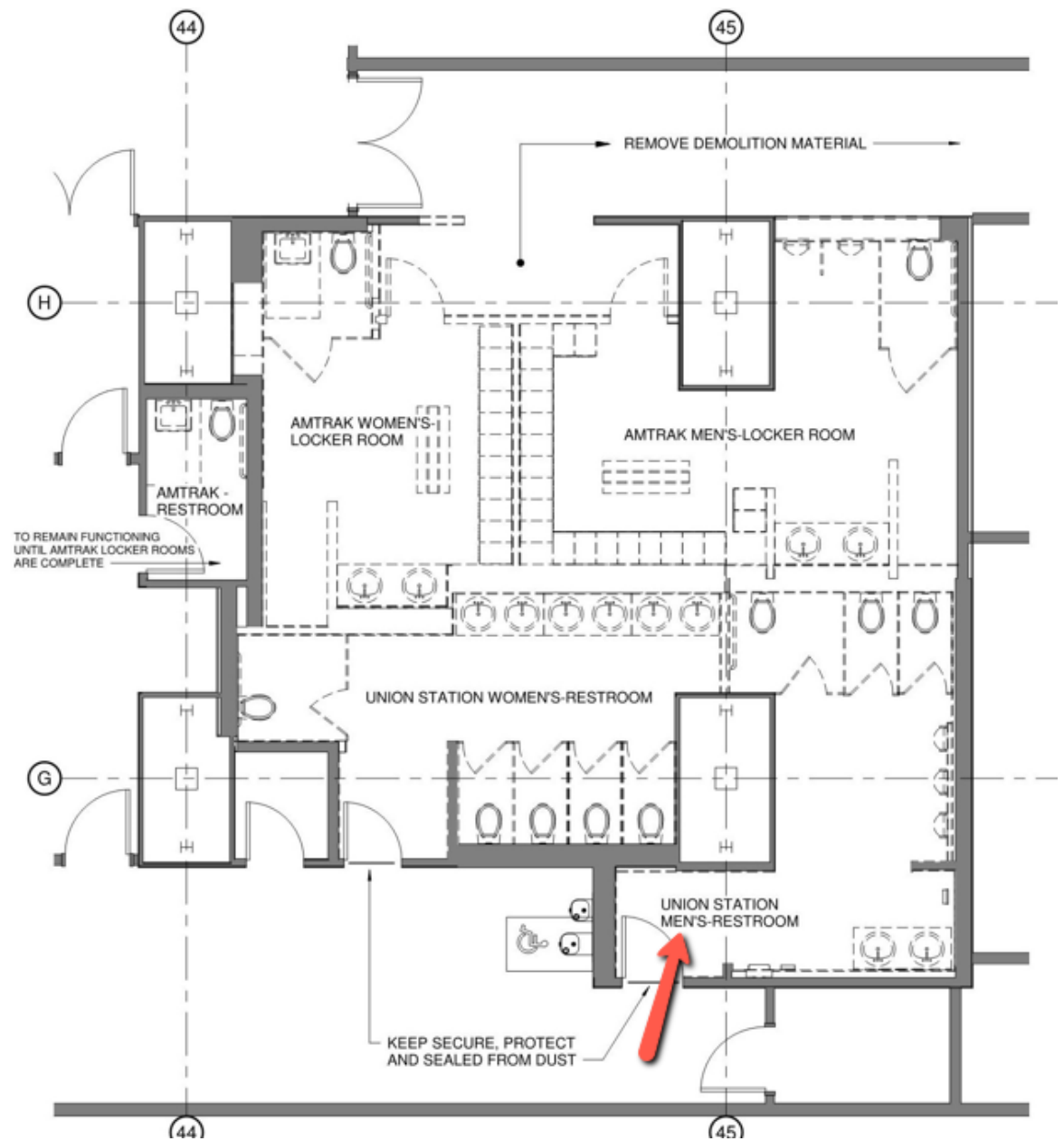
Public Restroom- Mens
