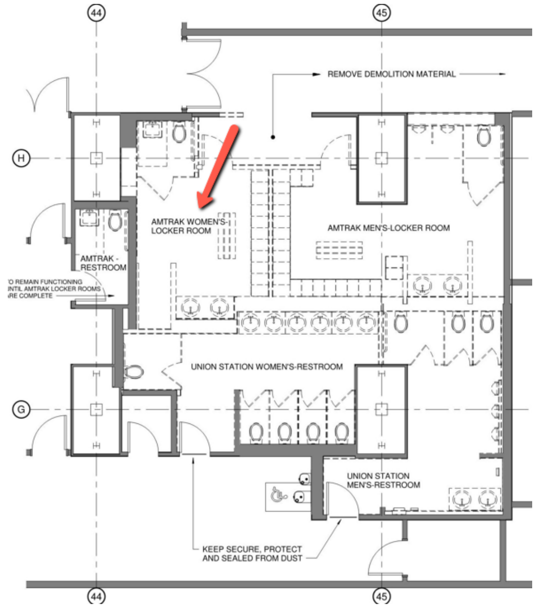
AMTRAK Womens Locker Room
