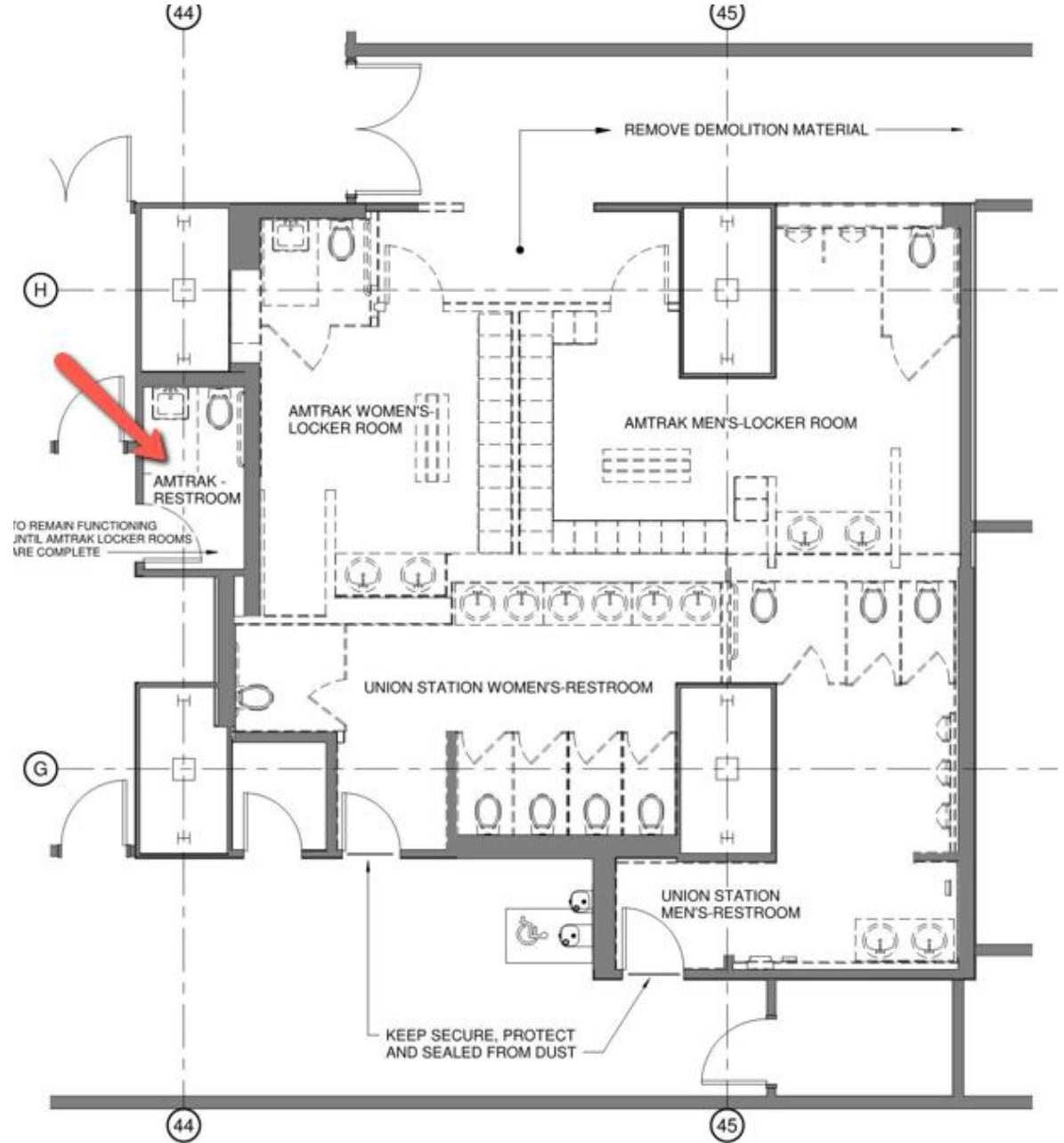
AMTRAK Single Restroom
