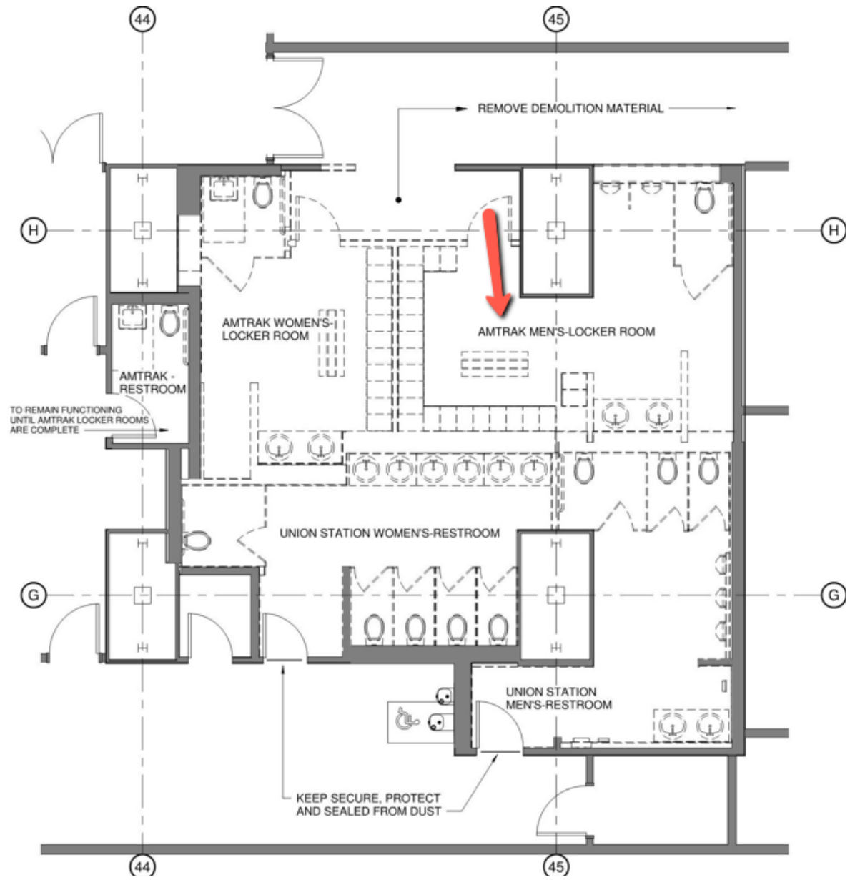
AMTRAK Mens Locker Room
