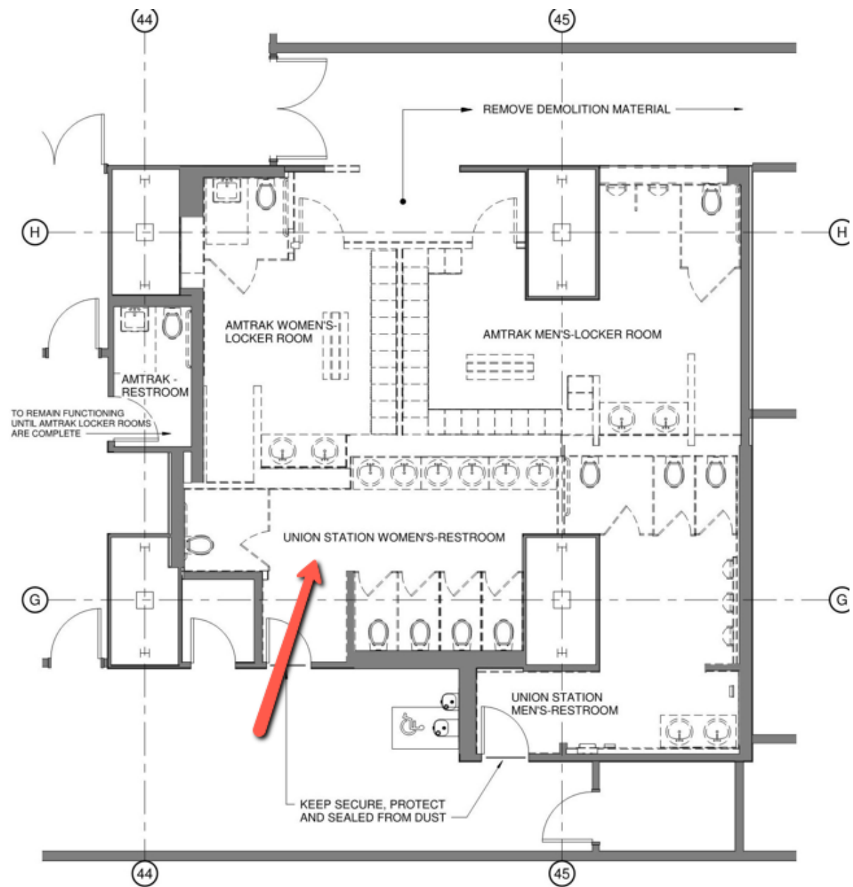
Public Restroom- Womens
